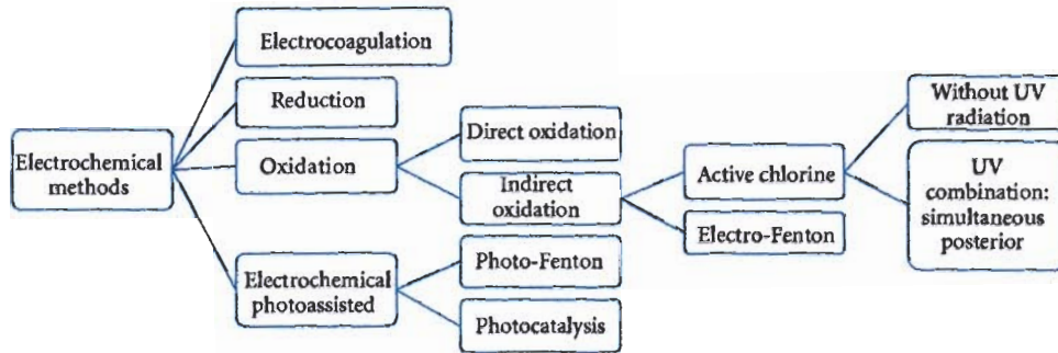
FIGURE 6: Electrochemical methods.
